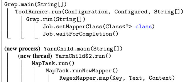
Figure 10: The call graph in Hadoop with RegexMapper.
